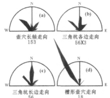
图 5 壶穴长轴、三角坑各边、三角坑长边、槽型壶穴走向(图中数字为样本数) Fig. 5 Directions of long axes of potholes, each edge and the longest edge of triangular pits, and groove holes
